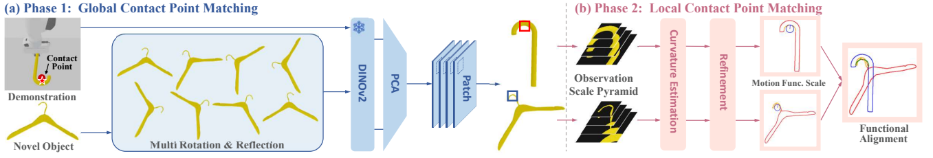
Fig. 3: Global and Local Contact Point Matching. The contact point matching process consists of two phases: (a) global matching using DINOv2 [44] features; (b) local matching involving multi-scale curvature estimation and refinements using irrelevant point suppression and convexity matching.
